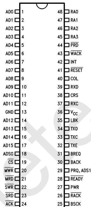
Dual-In-Line Package
